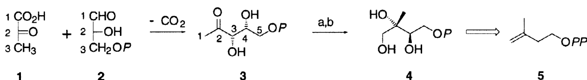
Fig. 1. Mevalonate-independent route for isoprenoid biosynthesis: a) rearrangement; b) reduction by NADPH.
