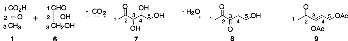
Fig. 2. Biosynthesis of laurencione 8 from pyruvate 1 and glyceraldehyde 6 and from 1-deoxy-D-xylulose 7 by bacterial cell-free systems.
