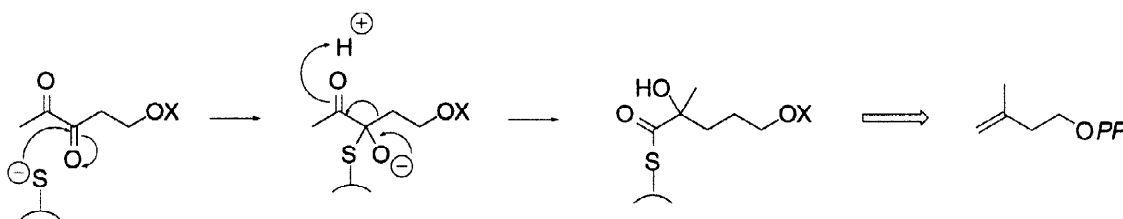
Fig. 3. Hypothetical biogenetic scheme for the formation of the isoprenic skeleton from laurencione (X = H or phosphate).
